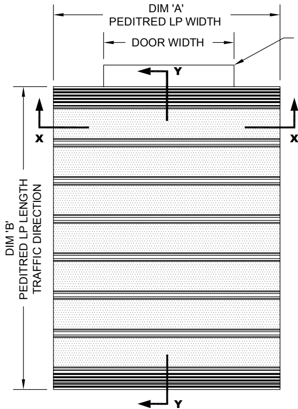
TYPICAL PLAN VIEW
