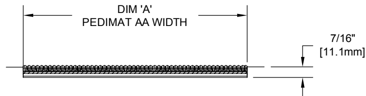
SECTION X-X
