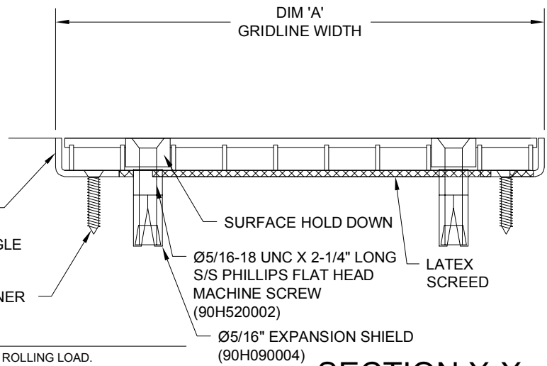
SECTION X-X
