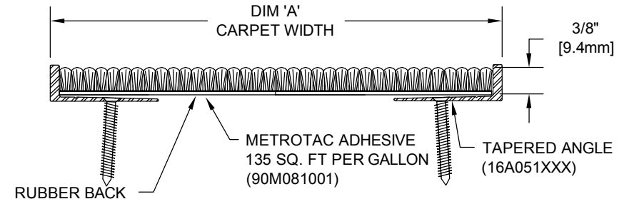
SECTION X-X
