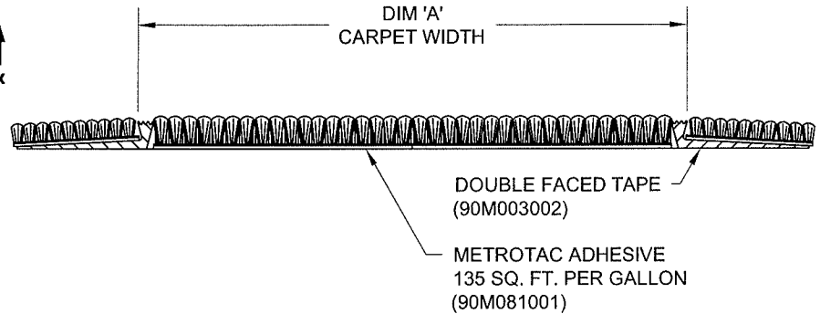
SECTION X-X
