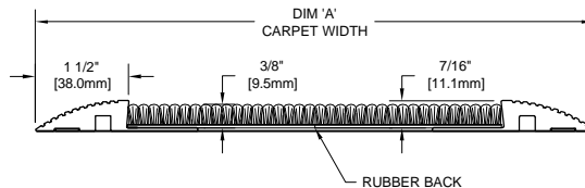
SECTION X-X
