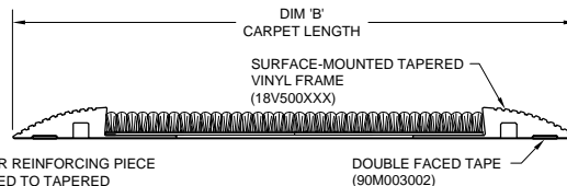
SECTION Y-Y
